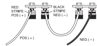
Figure 2. Series connection
