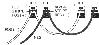
Figure 1. Parallel connection
